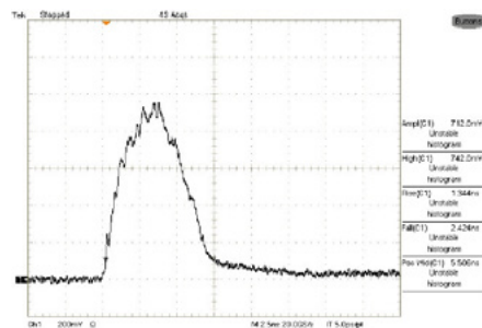
Typical optical output signal, driver designed for 5.5 ns pulses (time scaling 2.5 ns/div).
