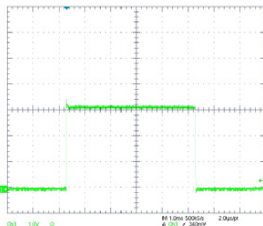
Figure: Current monitor output, scale: 100A/Div
