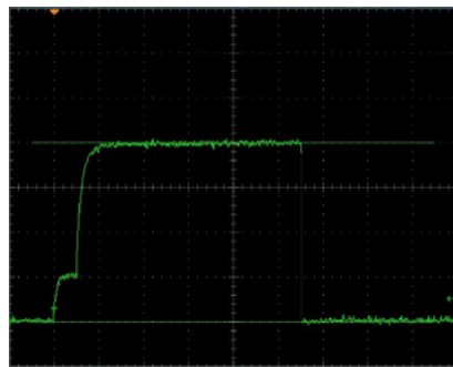
Figure: Output signal for a 50 µs / 50 A prepulse and 200 A / 500 µs main pulse
