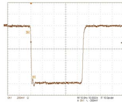
Figure: Current monitor output, scale: -0.4 A/Div
