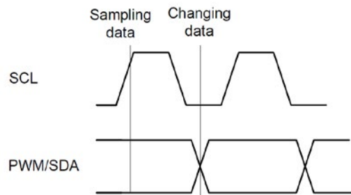
Figure 10. Bit transfer on SMBus.
