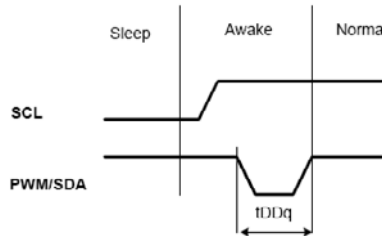
Figure 12. Exiting Sleep Mode.
