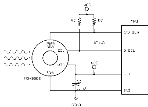
Figure 17. TSM SMBus connection.
