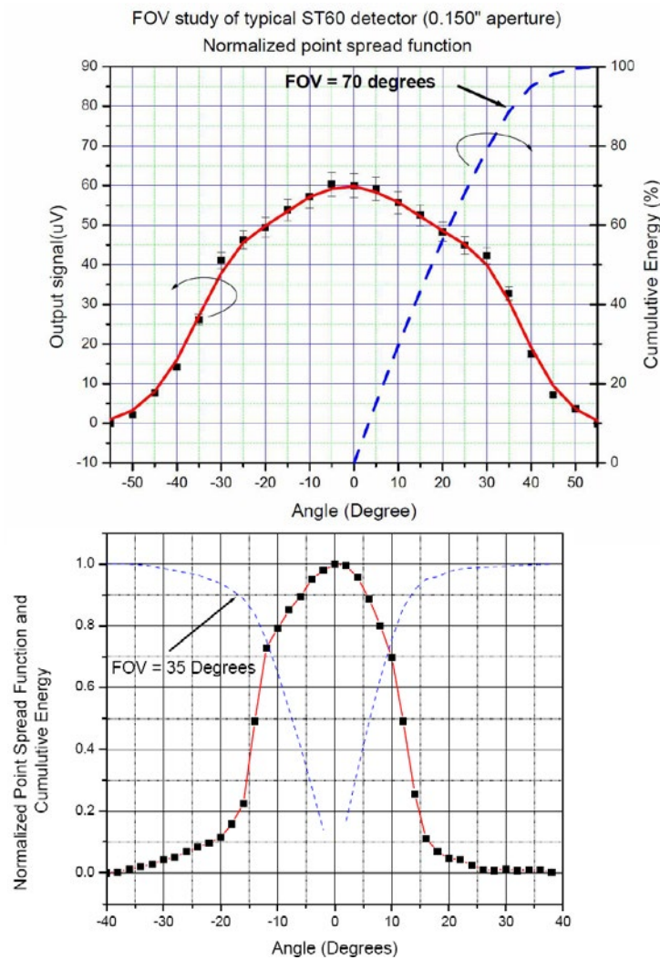
Figure 3. FOV for 70 and 35 degrees.
