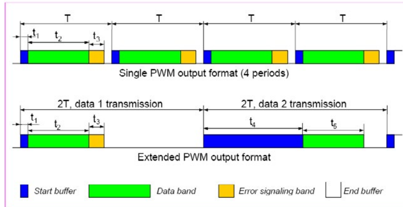
Figure 13. Pulse Width Modulation timing.
