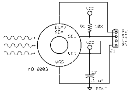
Figure 20. PWM output with SMBus available.
