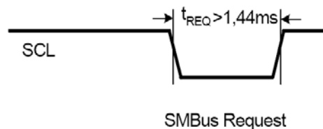
Figure 16. Request (switch to SMBus) condition.
