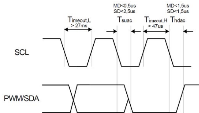
Figure 8. SMBus timing.
