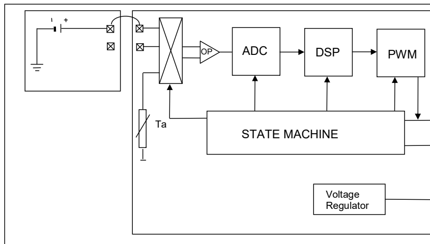
Figure 5. TSM Architecture.
