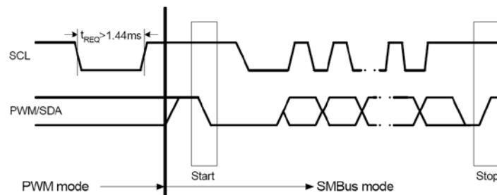
Figure 15. Switching from PWM mode to SMBus mode.
