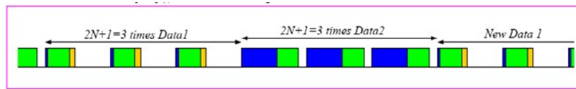
Figure 14. Extended PWM format with DUAL[5:1] = 0x01h (2 repetitions for each data).
