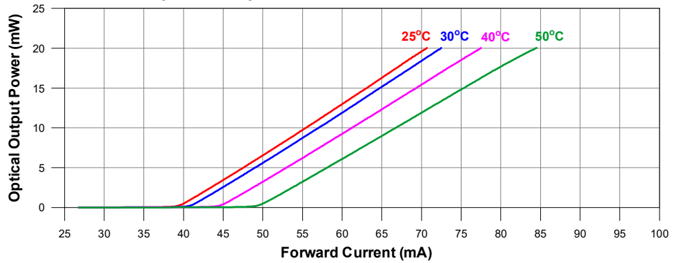
Optical Output Power v.s. Forward Current
