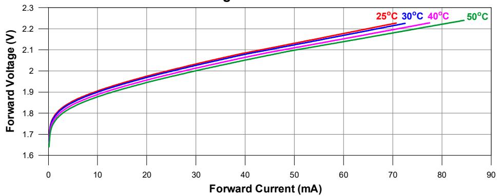
Forward Voltage v.s. Forward Current
