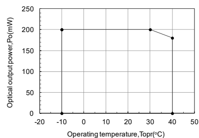
Figure.1 Optical output power vs. Operating temperature
