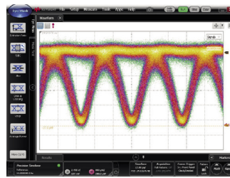
28 Gb/s Optical DPSK Eye Diagram
