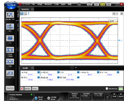
Output response Eye amplitude = 5.8 V pp
