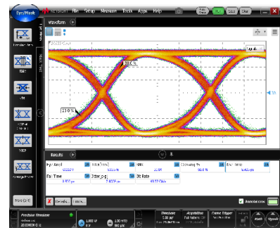
Output response Eye amplitude = 6 V pp
