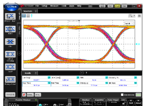
Data Rate = 10 Gb/s, V_{in} = 220 \text{ mV}_{pp}
