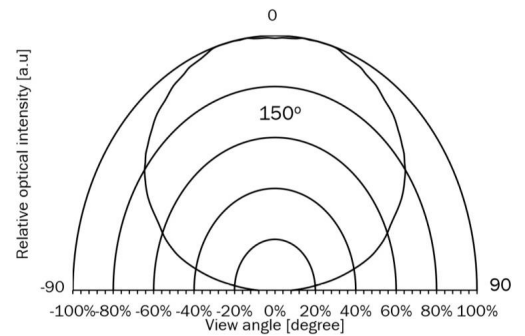
Fig 6. Far-field Emission Pattern
