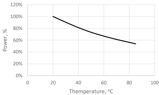
Fig 5. Relative Radiant Flux vs Ambient Temperature
