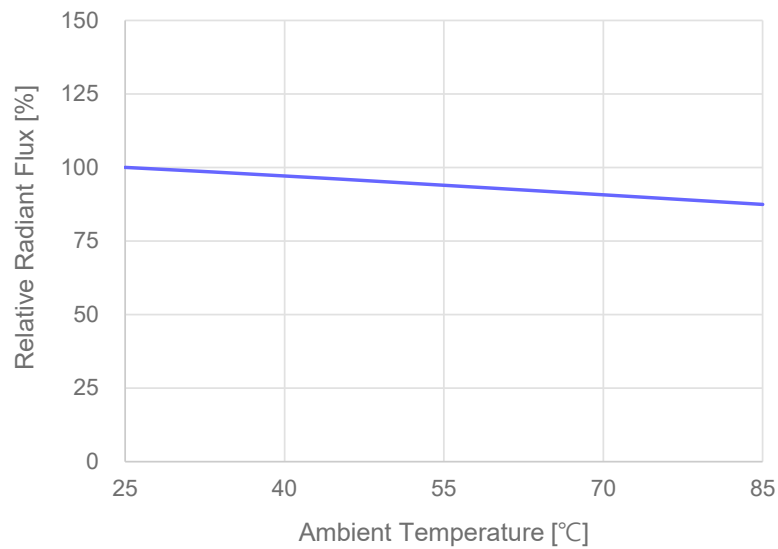
< Ambient Temperature vs. Relative Radiant flux >
