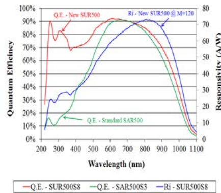
Figure 11. SUR500S8 quantum efficiency improvements
