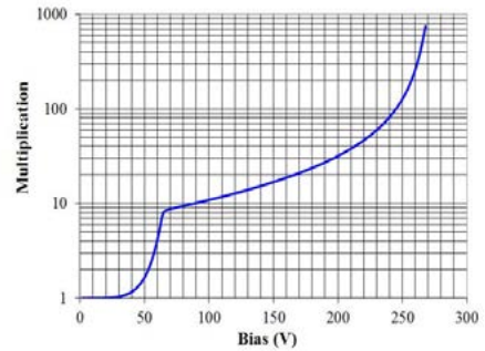
Figure 2. Typical multiplication gain characteristics measured on silicon RAPD
